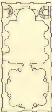
Fig. 263.—Plan of a Roman building. (From Bramantino's sketches in the Ambrosiana.)
